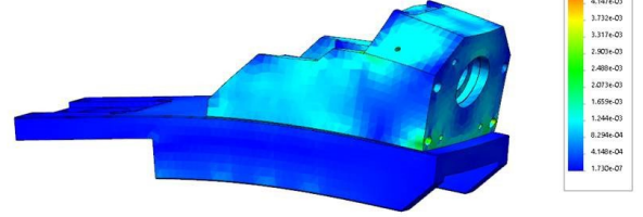
Finite Element Analysis strain results of 3 rd Axis (Y)
