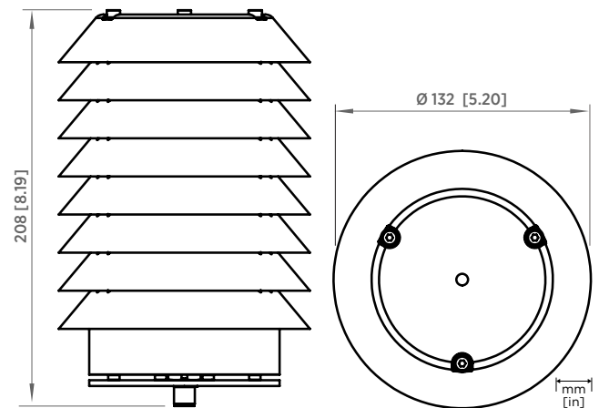
AQT420 dimensions
